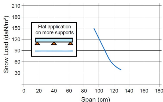
LOADING TABLE - LIGHTPIÙ WAVE 76/18 FLAT APPLICATION ON MORE SUPPORTS
