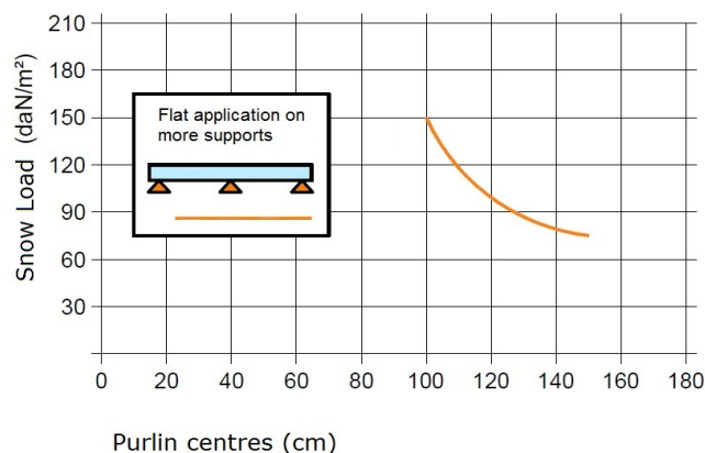
LOADING TABLE - SMARTPIU' GRECA 28/112 FLAT APPLICATION ON MORE SUPPORTS
